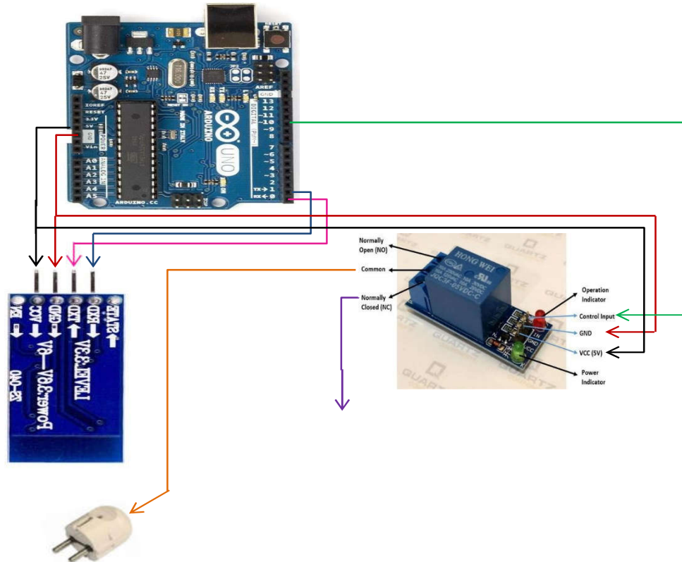
Gambar 1.1 Perancangan On/Off Neon box
